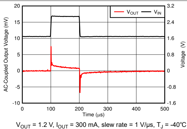
Figure 6-33. Line Transient
