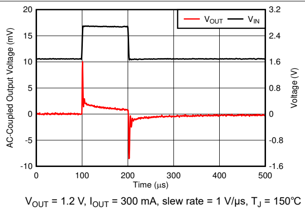
Figure 6-34. Line Transient
