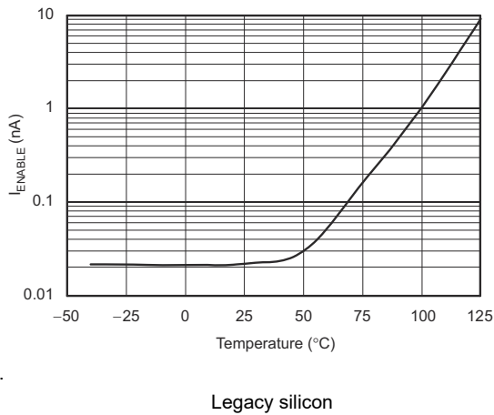
Figure 5-45. I_{ENABLE} vs Temperature
