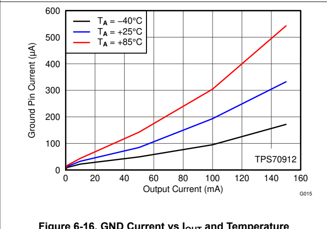
Figure 6-16. GND Current vs I_{OUT} and Temperature
