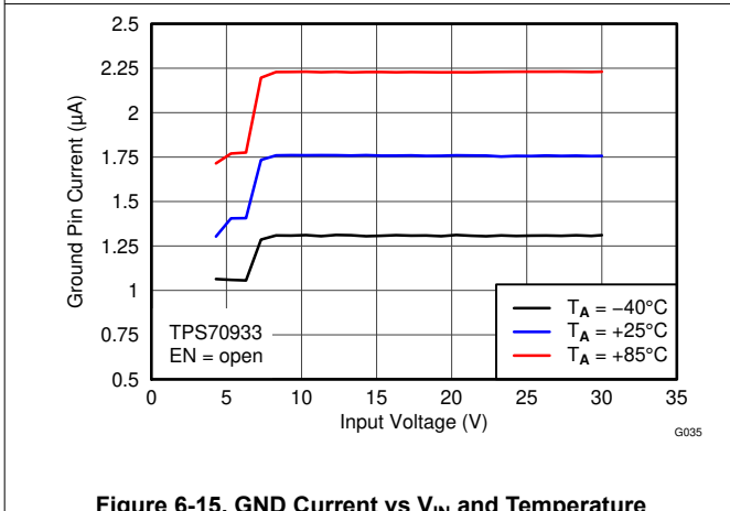
Figure 6-15. GND Current vs V_{IN} and Temperature
