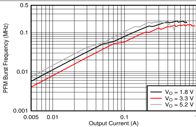
Figure 54. Burst Switching Frequency versus Output Current
