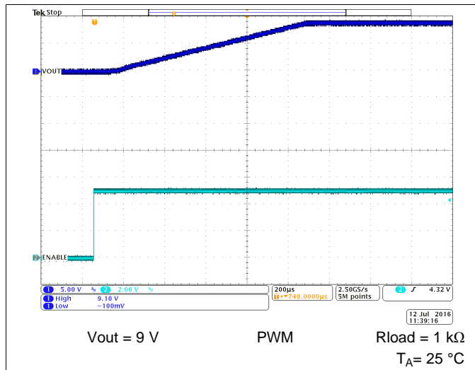
Figure 68. Start-Up Timing
