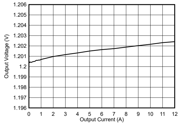
Figure 7-3. Load Regulation
