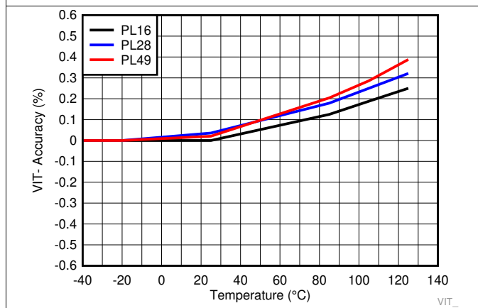
Figure 11. Negative-going Input Threshold Accuracy over Temperature for TPS3840PLXX
