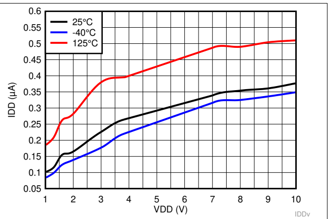
Figure 8. Supply Current vs Supply Voltage for TPS3840PL49
