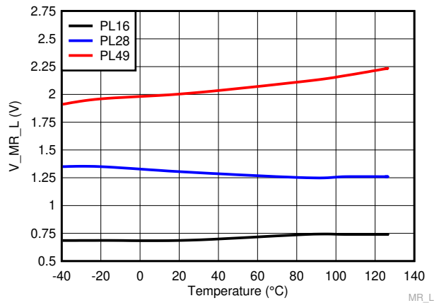
Figure 6-27. Manual Reset Logic Low Voltage Threshold over Temperature for TPS3840PLXX
