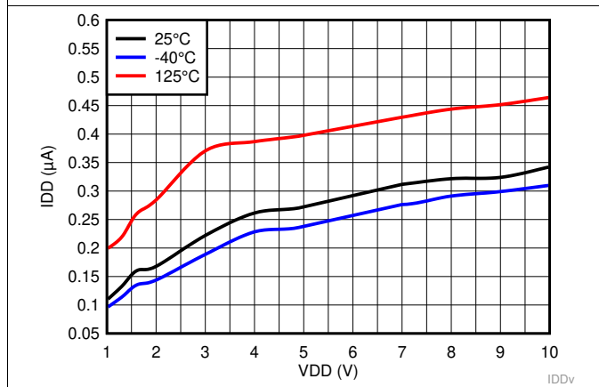
Figure 9. Supply Current vs Supply Voltage for TPS3840PH49
