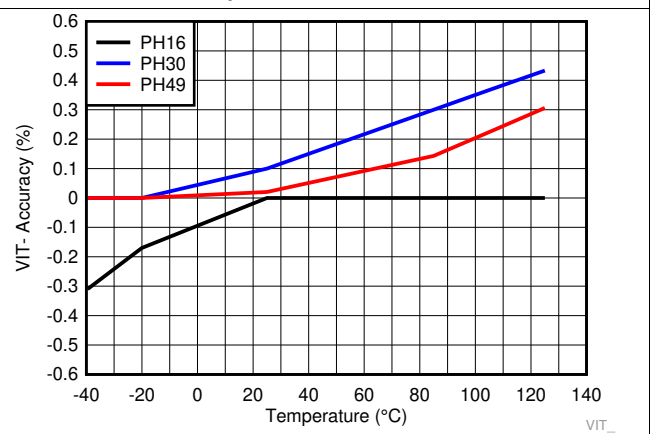
Figure 12. Negative-going Input Threshold Accuracy over Temperature for TPS3840PHXX
