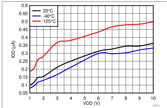
Figure 7. Supply Current vs Supply Voltage for TPS3840DL49
