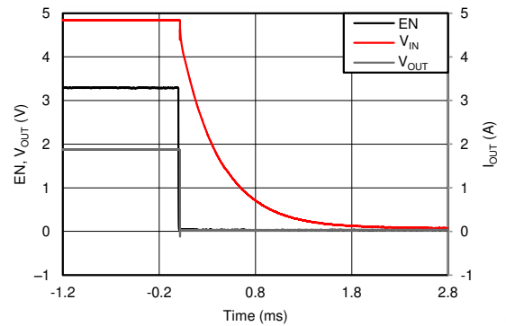
Figure 8-11. Turnoff Delay and Fall Time 150 \mu\text{F} // 2.5 \Omega
