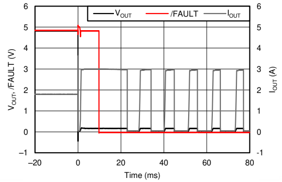
Figure 8-13. 2.5 Ω to Output Short Transient Response
