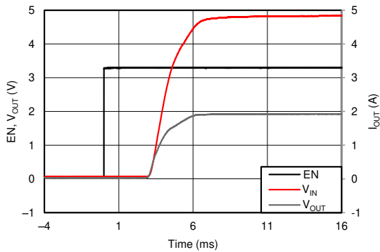
Figure 8-10. Turnon Delay and Rise Time 150 \mu\text{F} // 2.5 \Omega
