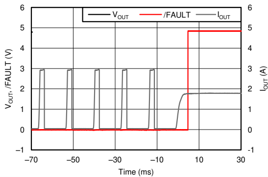
Figure 8-14. Output Short to 2.5-Ω Load Recovery Response
