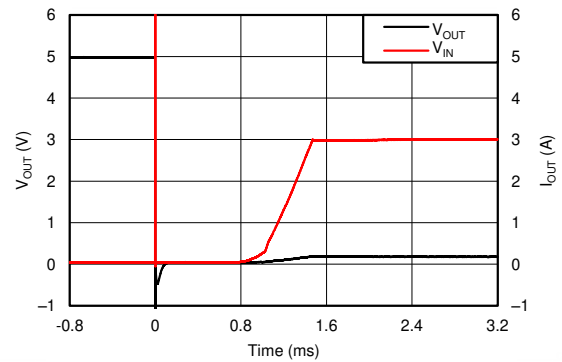
Figure 8-17. Hot-Short With 50 mΩ
