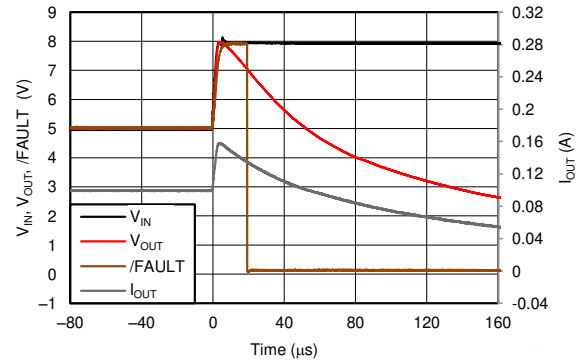
Figure 8-7. V_{IN} Step 5 V to 8 V with 4.7 \mu\text{F} // 100 \Omega
