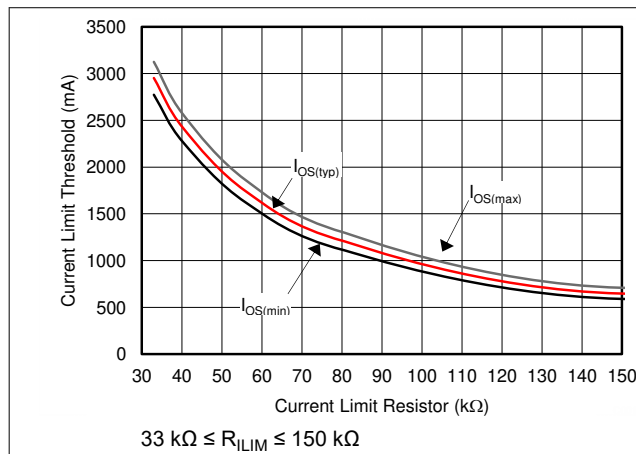
Figure 8-4. Current-Limit Threshold vs R_{ILIM} I
