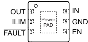
Figure 4-1. DRV Package 6-Pin WSON Top View
