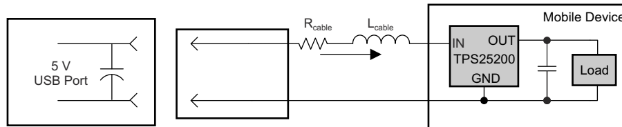
Figure 8-1. Hot Plug Into 5V USB port with Parasitic Cable Resistance and Inductance
