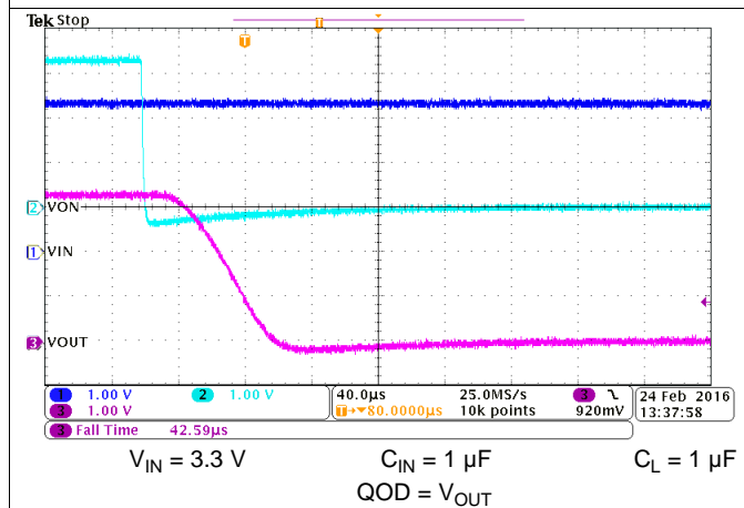
Figure 24. Fall Time ( t_F ) at V_{IN} = 3.3 V
