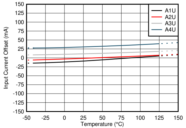
Figure 8-3. Offset Error Drift Across Temperature (U Variants)
