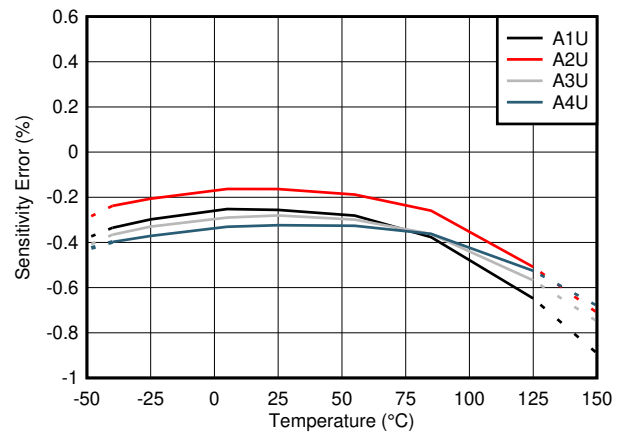
Figure 8-5. Sensitivity Drift Across Temperature (U Variants)
