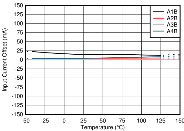
Figure 6-3. TMCS1101AxB Input Offset Current vs Temperature
