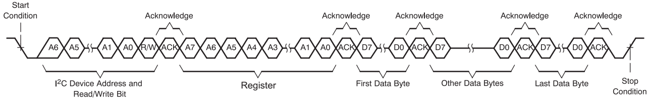
Figure 90. I 2 C Multiple-Byte Write Transfer
