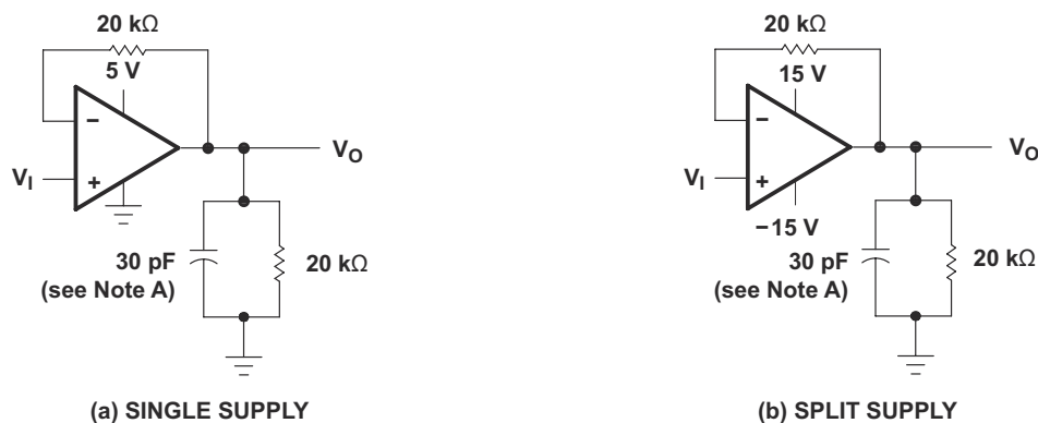
Figure 6-1. Slew-Rate Test Circuit
