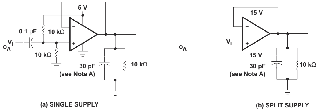
Figure 6-4. Small-Signal Pulse-Response Test Circuit
