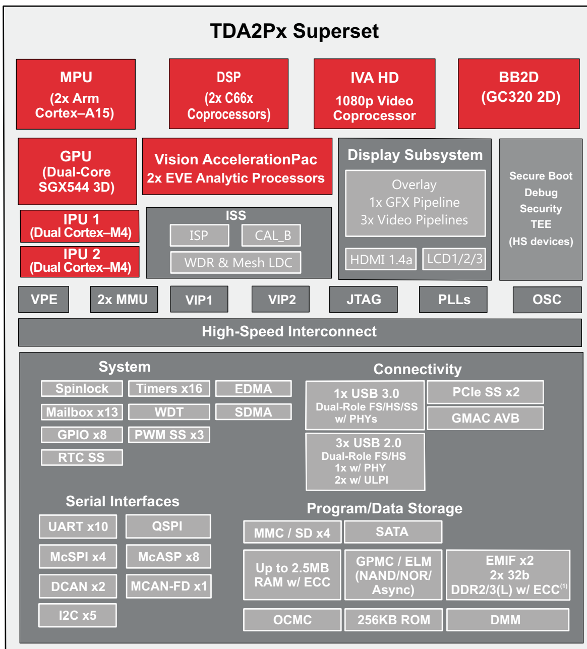
Figure 6-1. TDA2Px Block Diagram
