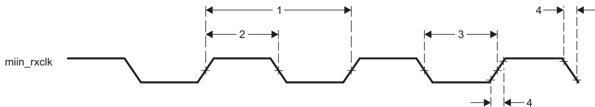
Figure 5-66. Clock Timing (GMAC Receive) - MII in Operation
