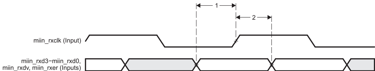
Figure 5-68. GMAC Receive Interface Timing MIIn Operation
