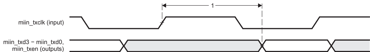
Figure 5-69. GMAC Transmit Interface Timing MIIn Operation
