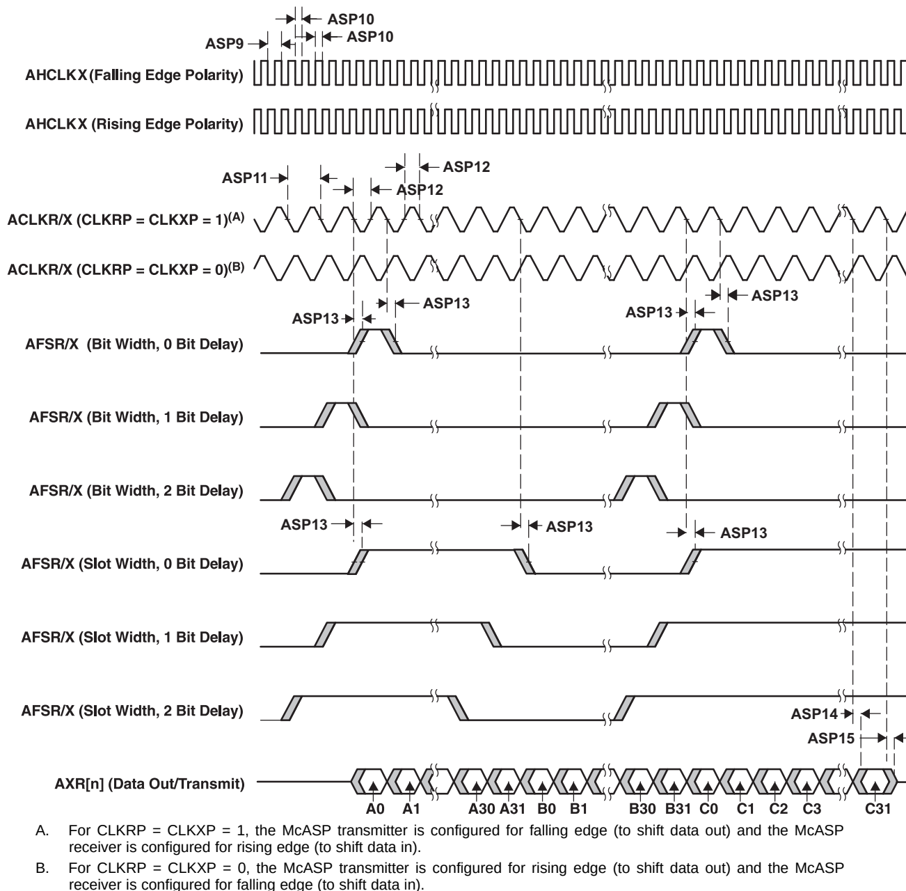
Figure 5-56. McASP Output Timing
