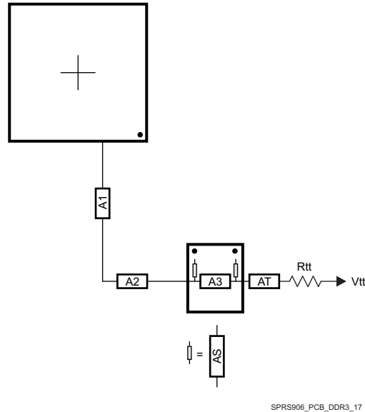
Figure 7-73. ADDR_CTRL Routing for Two Mirrored DDR3 Devices
