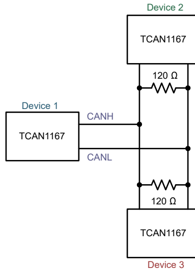
Figure 7-7. Three Node Example
