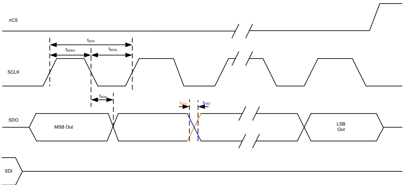
Figure 6-13. SPI AC Characteristic Read
