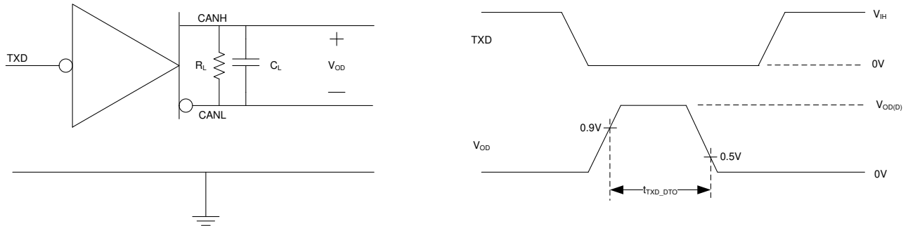
Figure 6-7. TXD Dominant Timeout Test Circuit and Measurement
