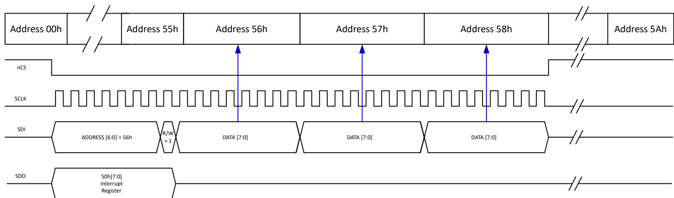
Figure 7-22. 32-bit SPI Burst Write
