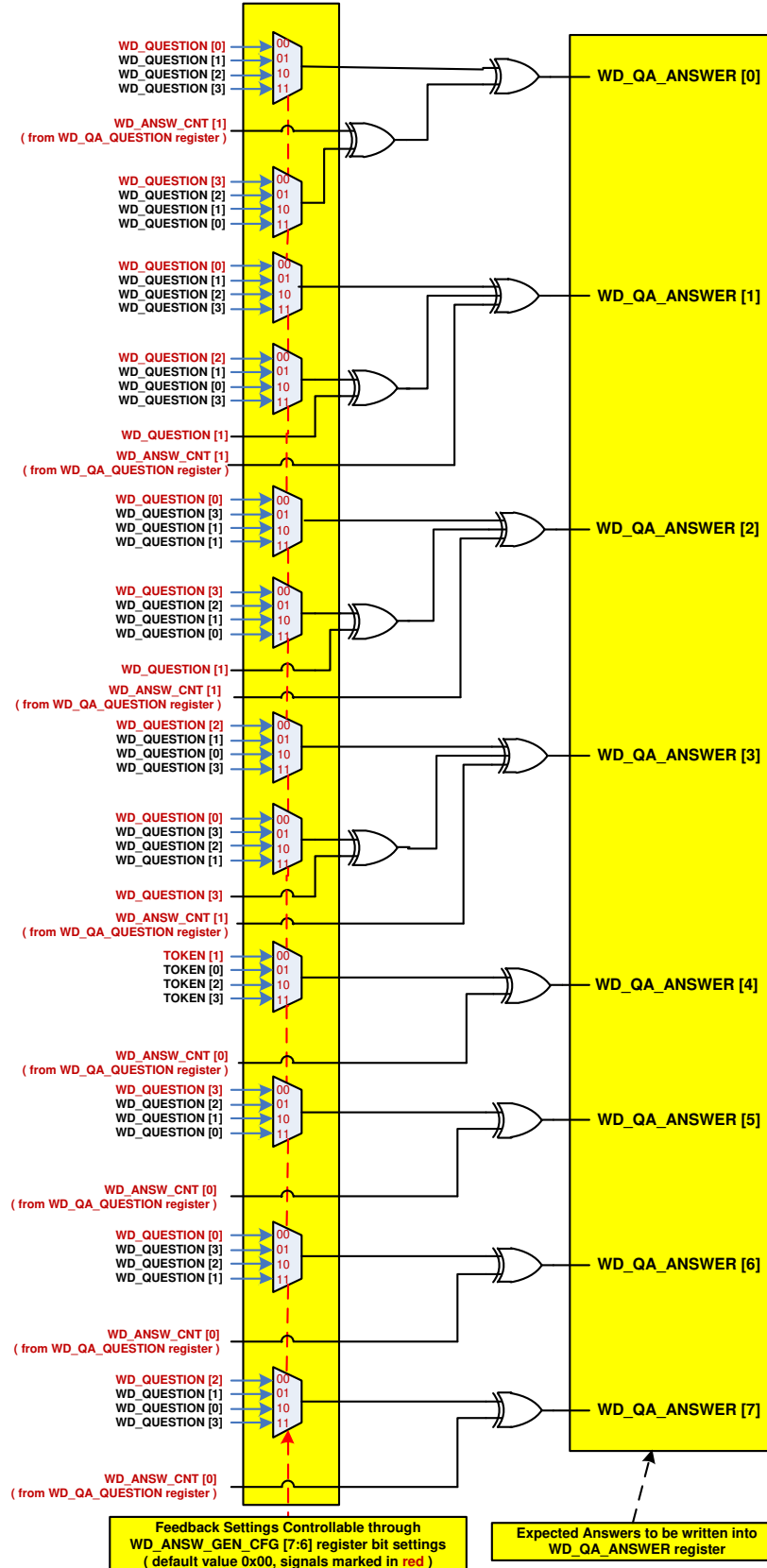
Figure 7-6. WD Expected Answer Generation
