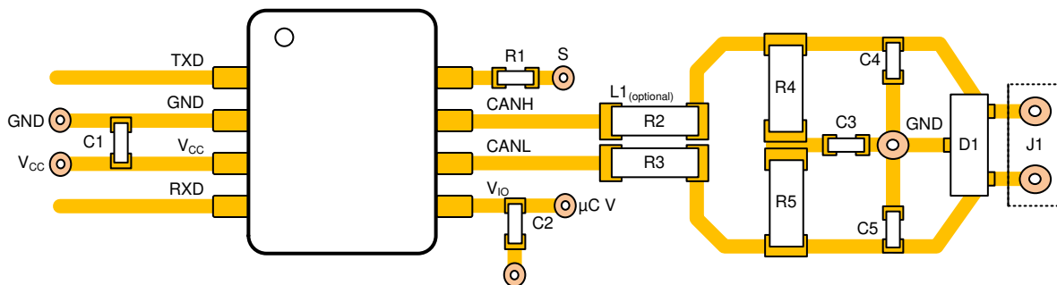
Figure 8-7. Layout Example
