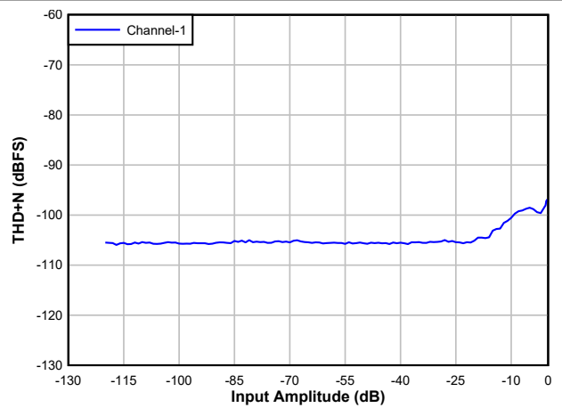
Single-ended output
