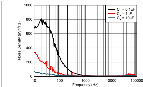
Figure 7-16. Noise Spectrum 10Hz to 100kHz ( V_{REF} = 2.5V )
