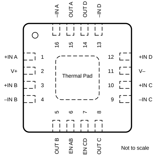
Not to scale Figure 5-8. OPA4392 RTE Preview Package, 16-Pin WQFN (Top View)
