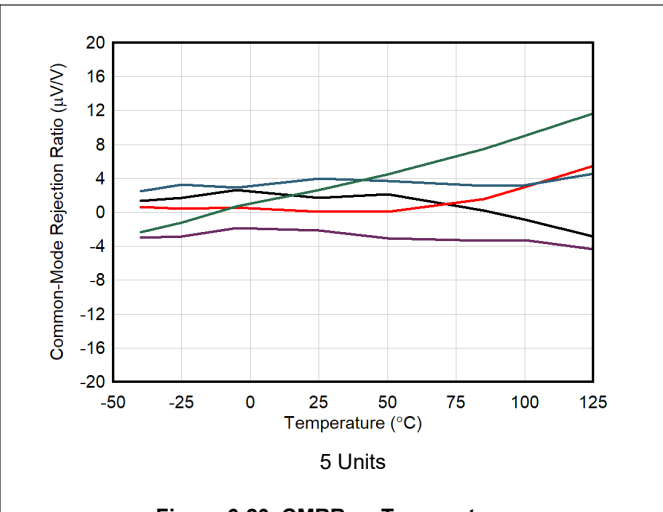
Figure 6-20. CMRR vs Temperature
