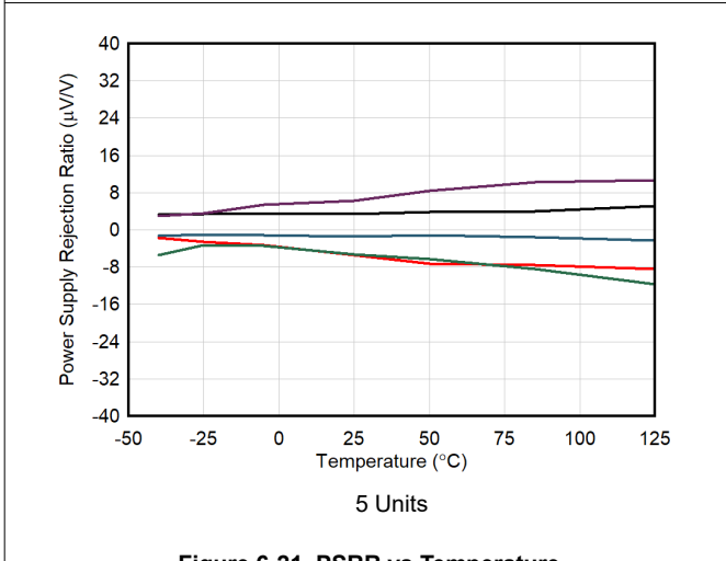
Figure 6-21. PSRR vs Temperature
