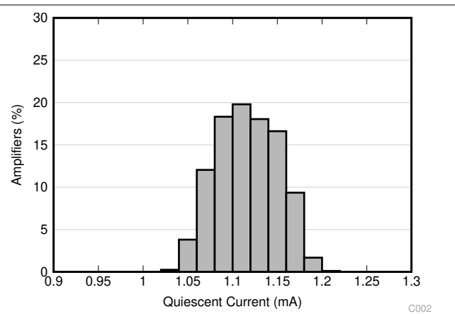
Figure 6-8. Quiescent Current Distribution
