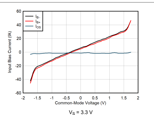
Figure 6-12. Input Bias Current vs Common-Mode Voltage
