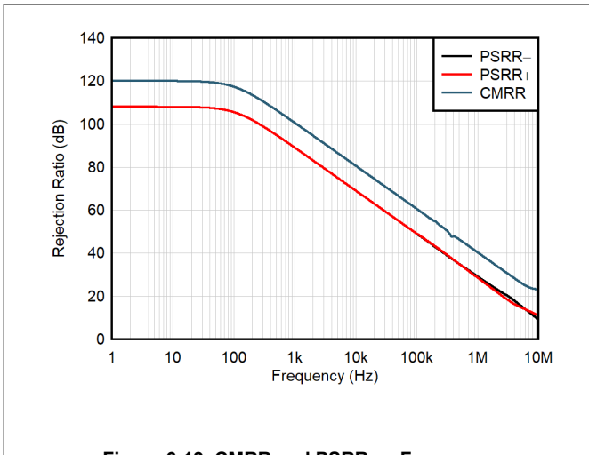
Figure 6-19. CMRR and PSRR vs Frequency
