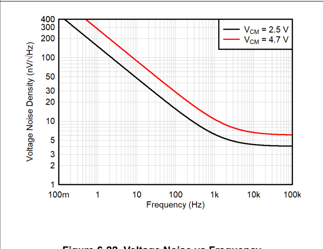
Figure 6-22. Voltage Noise vs Frequency
