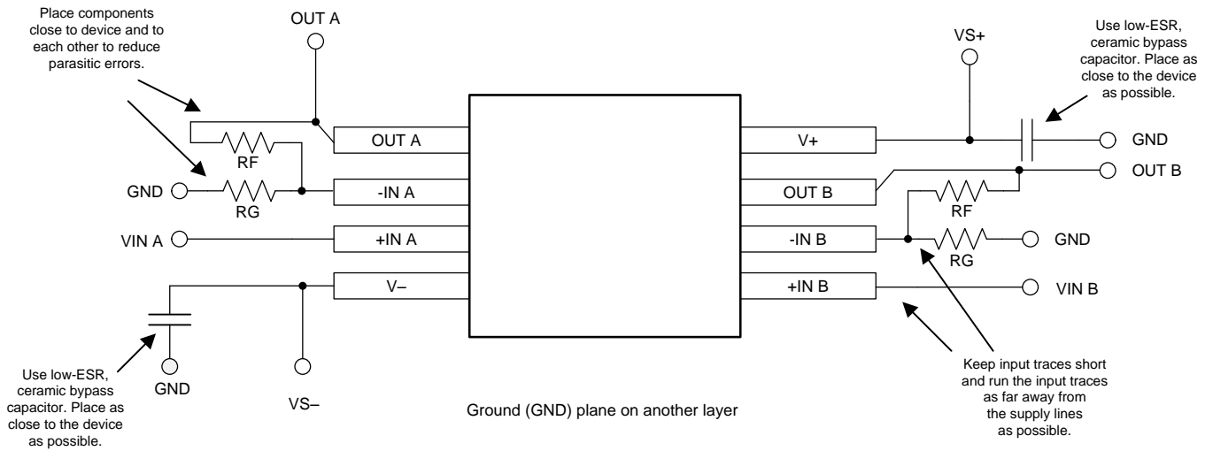
Figure 57. Layout Example
