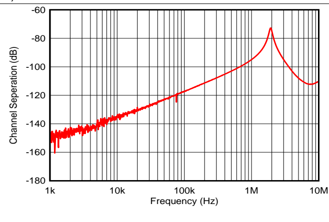
Figure 26. Channel Separation vs Frequency
