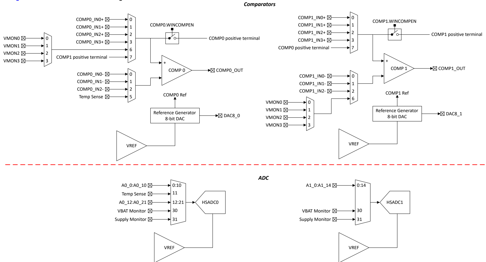
Figure 8-2. Device Analog Connection
