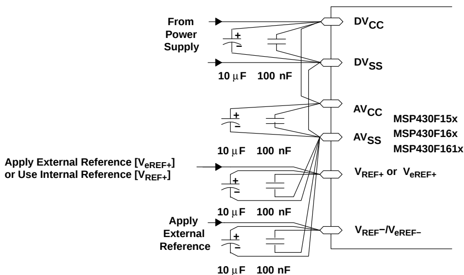
Figure 17. Supply Voltage and Reference Voltage Design V_{REF-}/V_{REF-} External Supply
