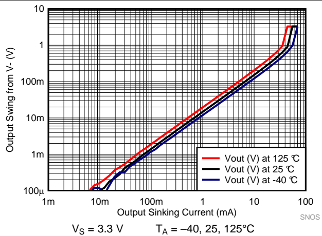
Figure 30. Output Swing vs. Sinking Current, 3.3\text{ V}
