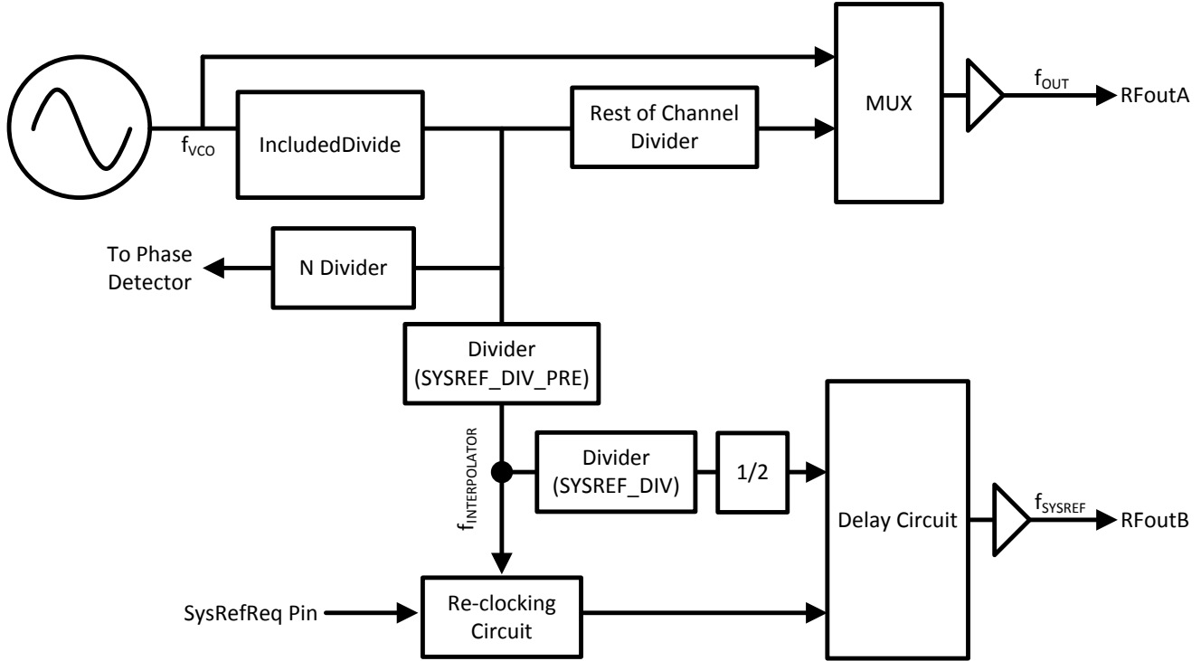
Figure 6-9. SYSREF Setup
