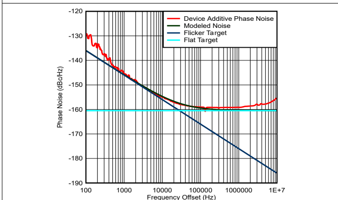
Figure 5-6. Flicker Noise
