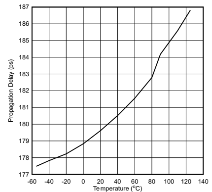
Figure 5-18. Propagation Delay
