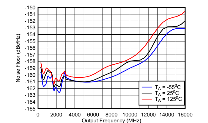
Figure 5-7. Noise Floor in Buffer Mode
