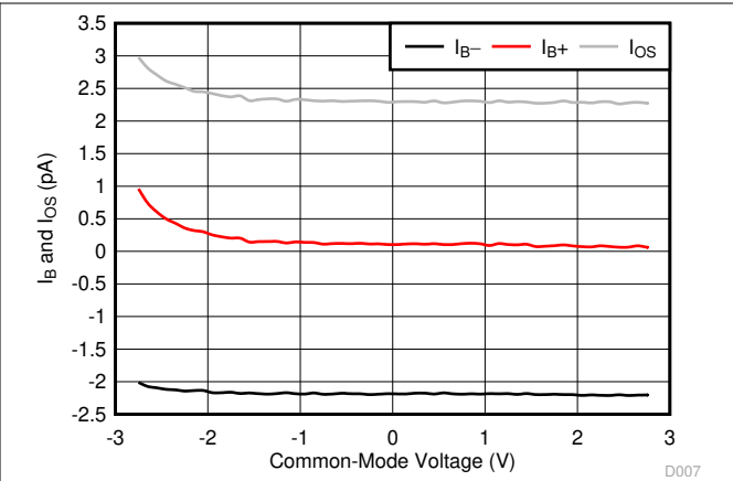
Figure 5-2. I_B and I_{OS} vs Common-Mode Voltage
