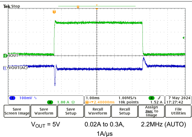
Figure 8-14. Load Transient
