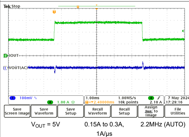
Figure 8-15. Load Transient
