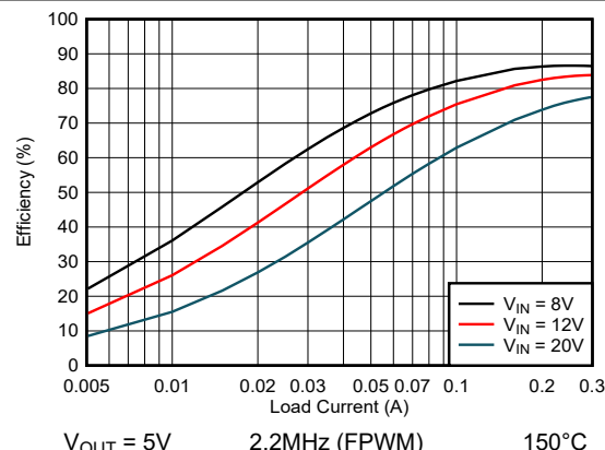
Figure 8-11. Efficiency
