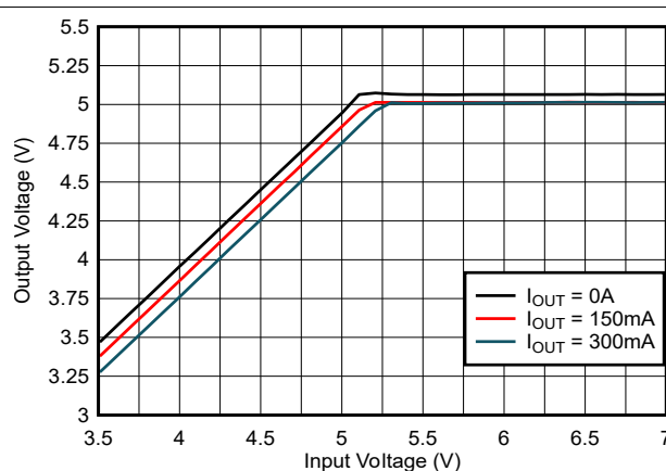
Figure 8-13. Dropout
