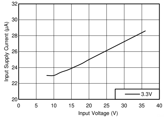
Figure 9-26. Input Supply Current
