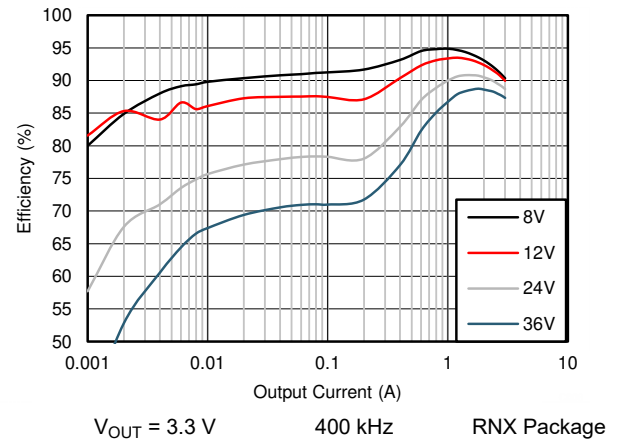
Figure 9-14. Efficiency
