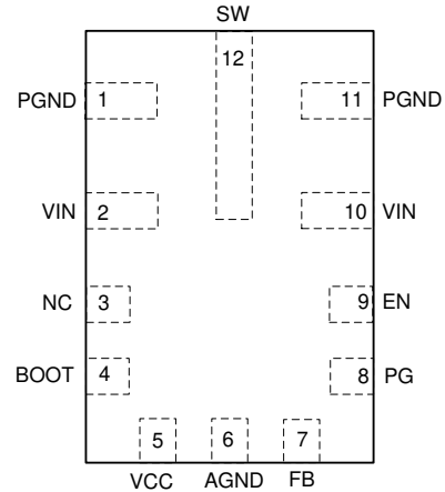
Figure 6-2. RNX Package 12-Pin VQFN Top View
