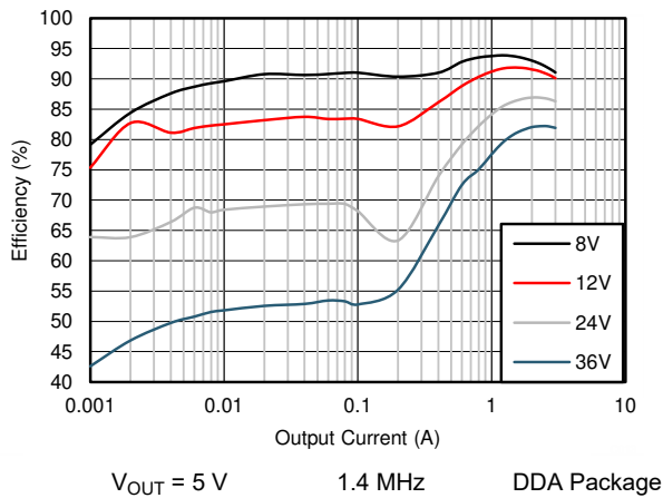
Figure 9-9. Efficiency
