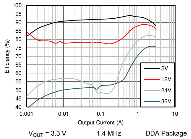
Figure 9-10. Efficiency
