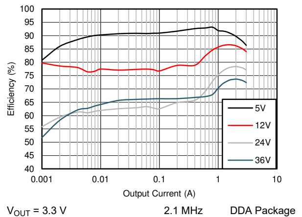
Figure 9-12. Efficiency
