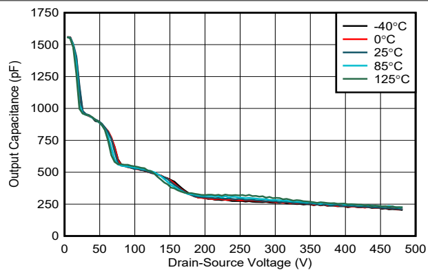
Figure 5-8. Output Capacitance vs Drain-Source Voltage
