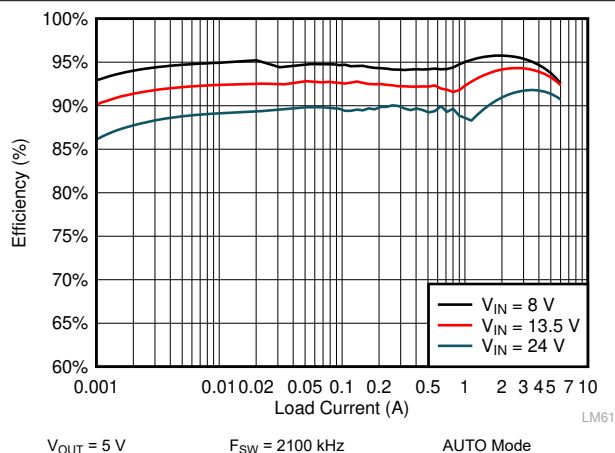
Figure 10-11. LM61460-Q1 Efficiency
