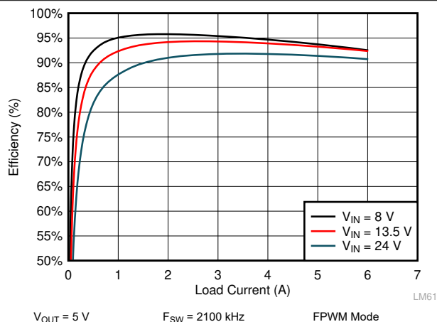
Figure 10-12. LM61460-Q1 Efficiency
