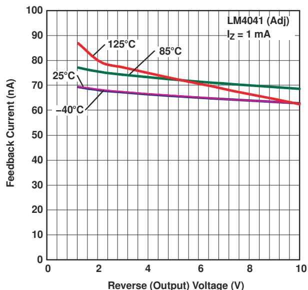
Figure 5-6. Feedback Current vs Reverse (Output) Voltage (for Different Temperatures)
