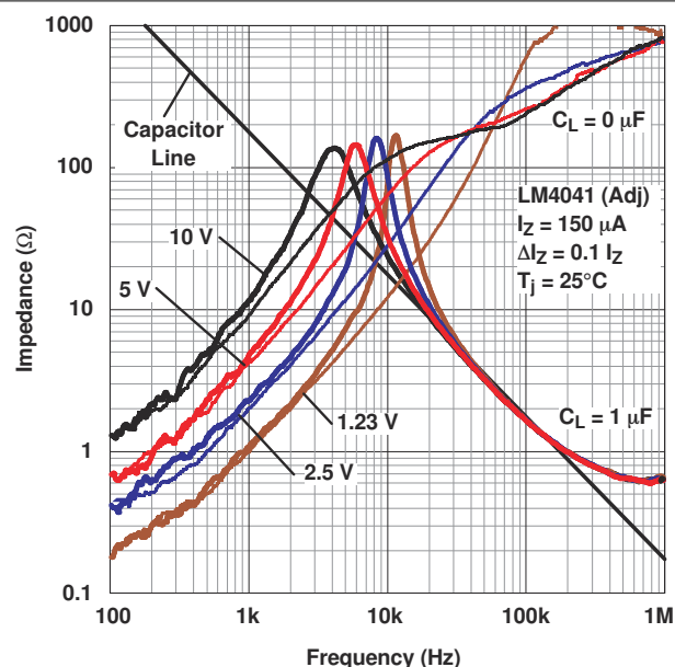
Figure 5-8. Output Impedance vs Frequency
