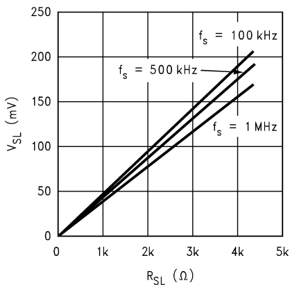
Figure 5-17. Compensation Ramp vs Compensation Resistor
