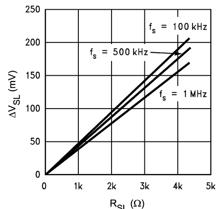
Figure 6-5. External Slope Compensation \Delta V_{SL} vs R_{SL}
