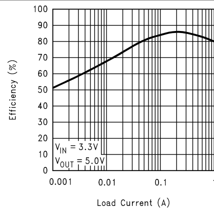
Figure 5-12. Efficiency vs Load Current (3.3-V Input and 5-V Output)
