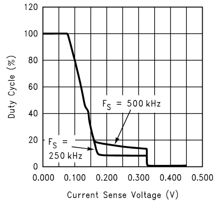
Figure 5-19. Duty Cycle vs Current Sense Voltage
