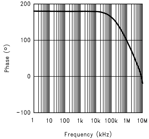
Figure 5-14. Error Amplifier Phase
