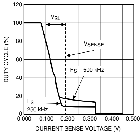
Figure 7-4. Current Sense Voltage vs Duty Cycle
