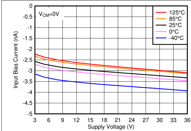
Figure 2-15. Input Bias Current vs. Supply Voltage
