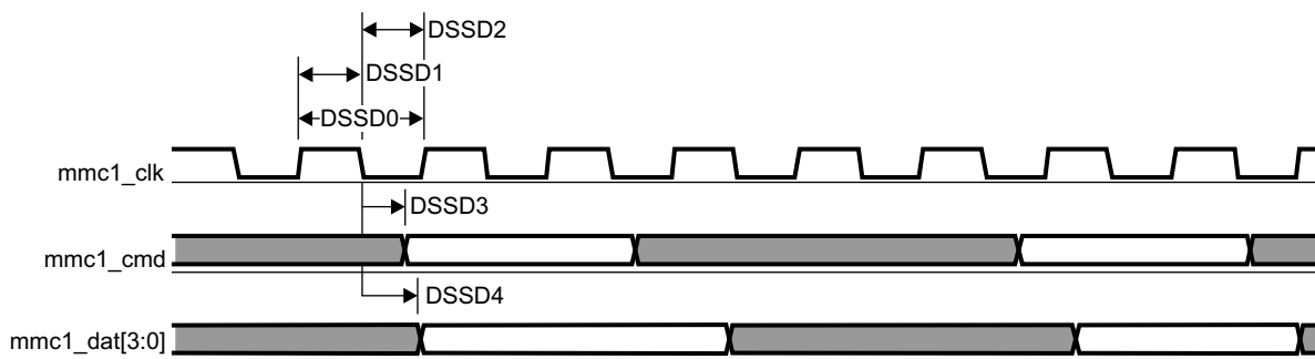
Figure 5-79. MMC/SD/SDIO in - Default Speed - Transmitter Mode
