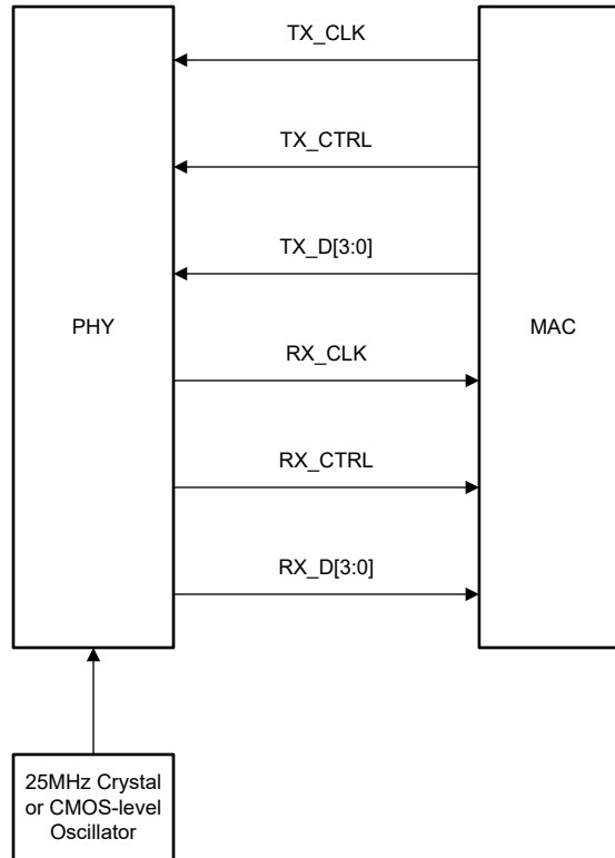
Figure 7-13. RGMII Connections
