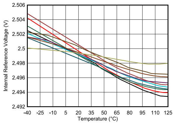
Figure 5-45. Internal Reference Voltage vs Temperature
