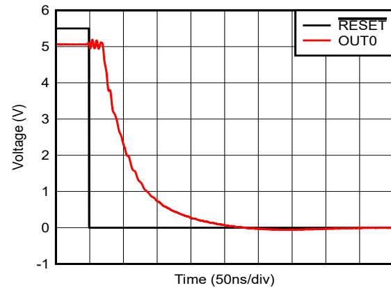
Figure 5-34. Glitch Impulse, Falling Edge
