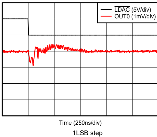
Figure 5-35. Glitch Impulse, Rising Edge
