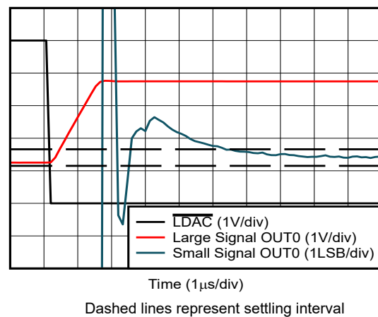
Figure 5-32. Full-Scale Settling Time, Rising Edge
