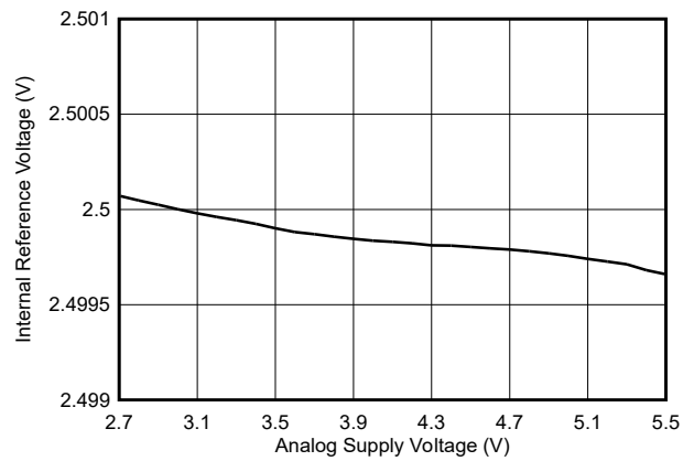
Figure 5-46. Internal Reference Voltage vs Supply Voltage
