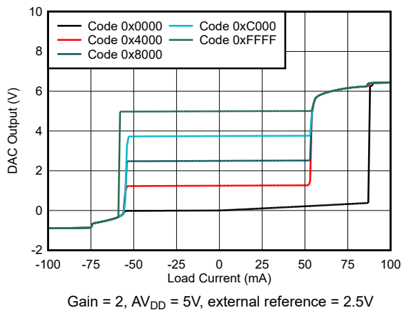
Figure 5-31. Source and Sink Capability
