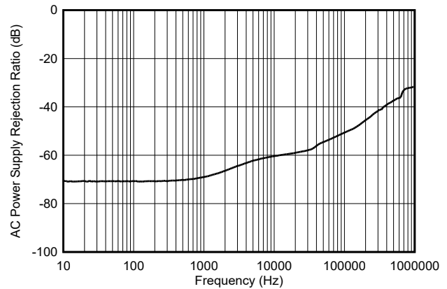
DAC code at full scale, V_{DD} = 5\text{V} + 200\text{mV}_{PP}
