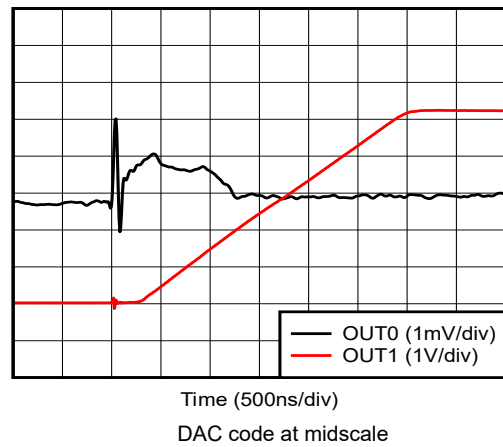
Figure 5-40. Channel-to-Channel Crosstalk
