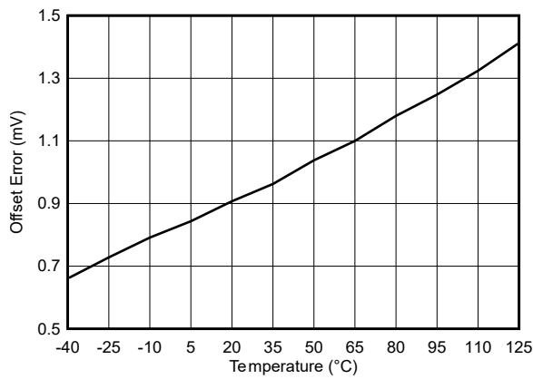
Figure 5-9. Offset Error vs Temperature
