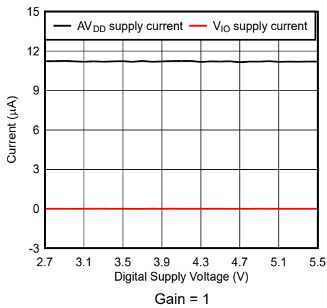
Figure 5-27. Power-Down Current vs V_{IO}
