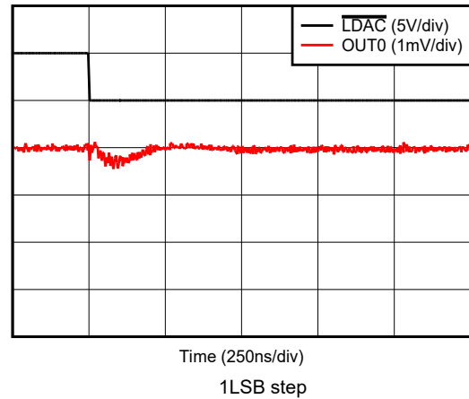
Figure 5-34. Glitch Impulse, Falling Edge
