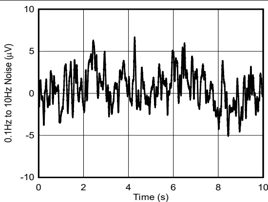
DAC code at midscale, gain = 2, external reference = 2.5V
