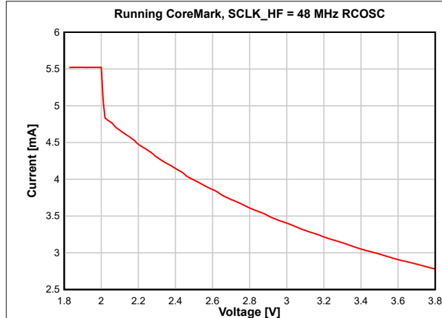
Figure 8-4. Active Mode (MCU) Current vs. Supply Voltage (VDD5)
