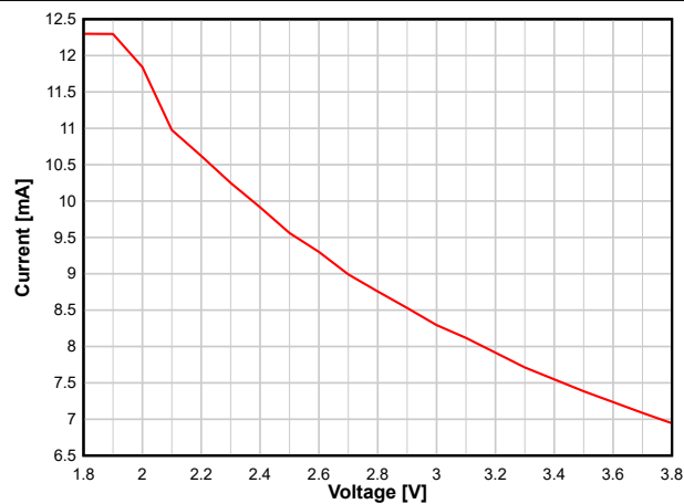
Figure 8-10. TX Current vs. Supply Voltage (VDDSD) (BLE 1 Mbps, 2.44 GHz, 0 dBm)
