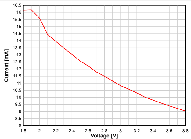
Figure 8-11. TX Current vs. Supply Voltage (VDDSD) (BLE 1 Mbps, 2.44 GHz, +5 dBm)
