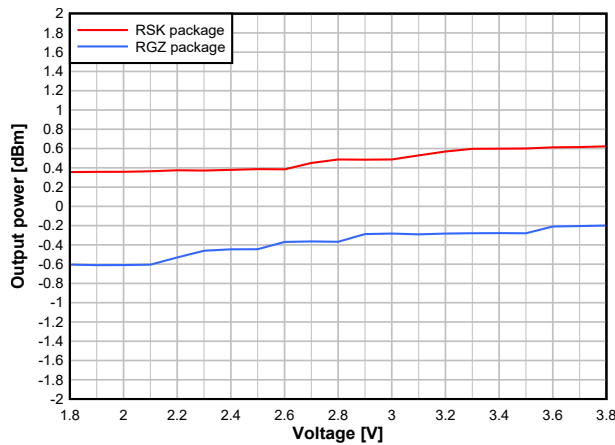
Figure 8-29. Output Power vs. Supply Voltage (VDD5) (BLE 1 Mbps, 2.44 GHz, 0 dBm)
