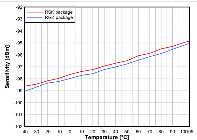
Figure 8-19. Sensitivity vs. Temperature (BLE 1 Mbps, 2.44 GHz)
