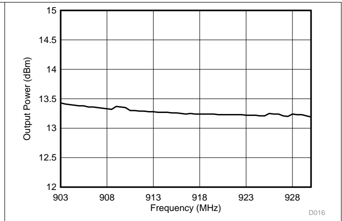
Figure 5-26. TX Maximum Output Power, 902 MHz to 928 MHz
