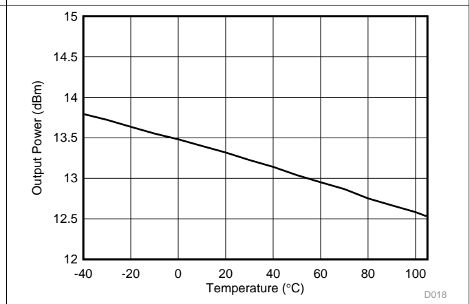
Figure 5-28. TX Maximum Output Power vs Temperature, 915 MHz
