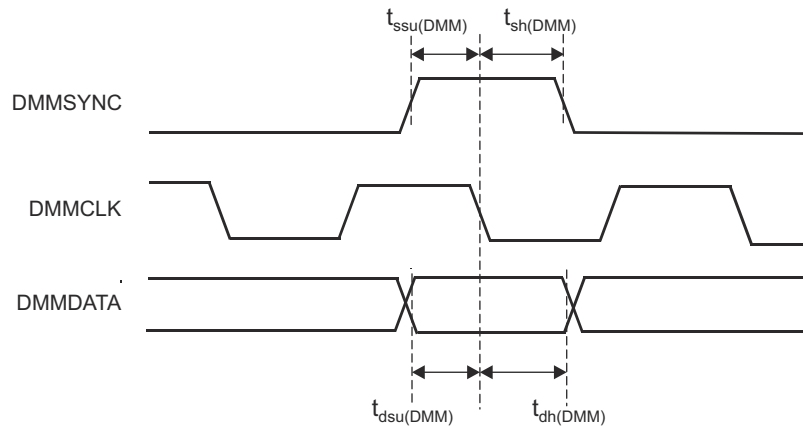
Figure 7-19. DMMDATA Timing
