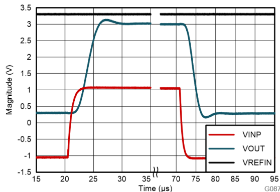
Figure 8-4. Step Response of the AMC0380R-Q1
