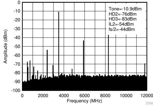
Figure 4-148. TX Single Tone (-12dBFS) Output Spectrum at 3.5GHz (0- f_{DAC} )
