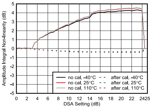
Figure 4-426. RX Amplitude Integrated Nonlinearity at 8.1GHz
