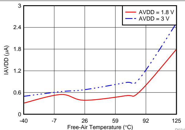
Figure 30. Analog Input Current in Autonomous modes with nCLK
