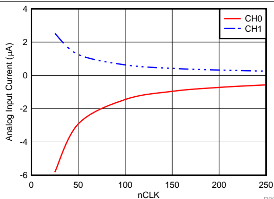
Figure 30. Analog Input Current in Autonomous modes with nCLK
