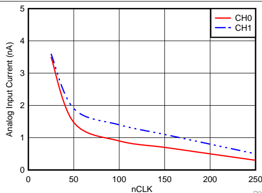
Figure 31. Analog Input Current in Autonomous modes with nCLK
