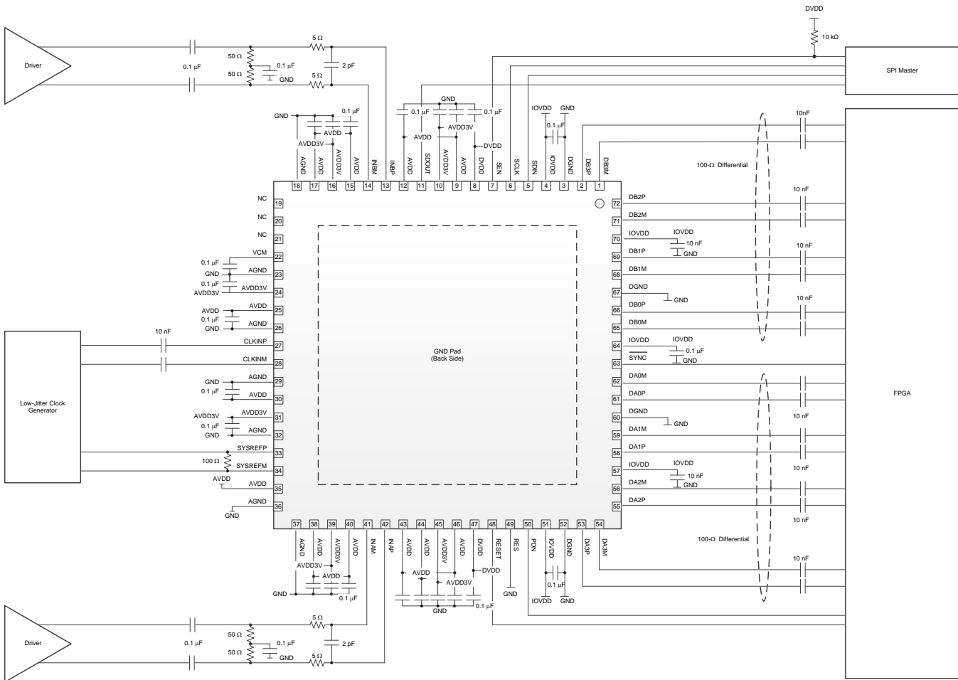
Figure 131. AC-Coupled Receiver
