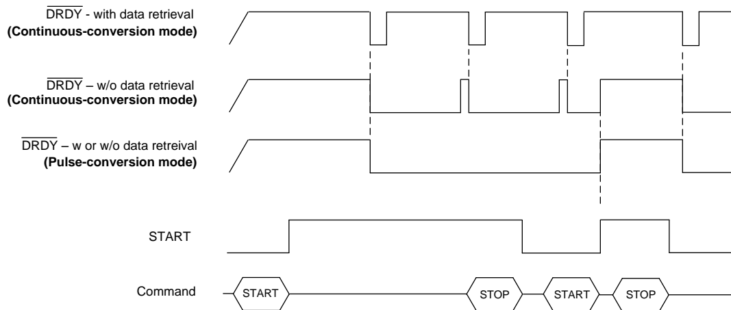
Figure 79. \overline{DRDY} Operation
