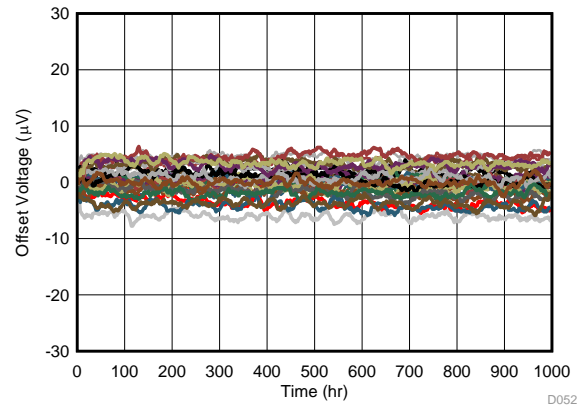
Figure 25. Offset Voltage Drift Distribution
