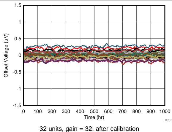
Figure 28. Offset Voltage Long-Term Drift
