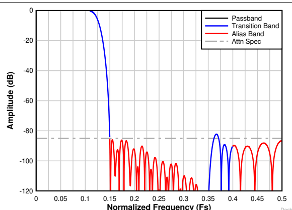
Figure 7-29. Decimation by 4 complex frequency response
