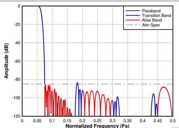
Figure 7-31. Decimation by 8 complex frequency response
