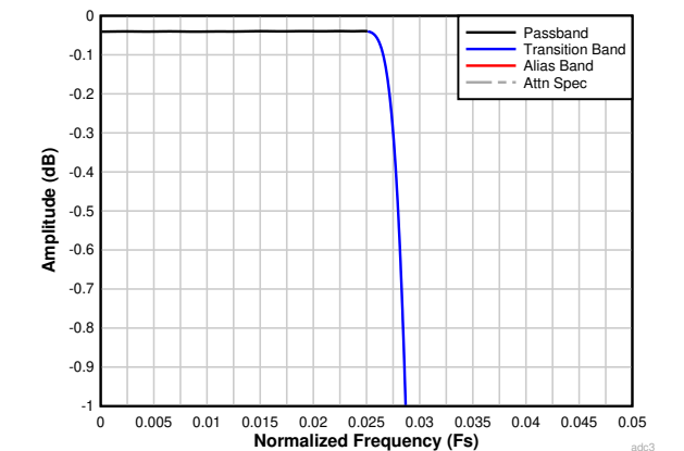
Figure 7-26. Decimation by 16 Passband Ripple Response
