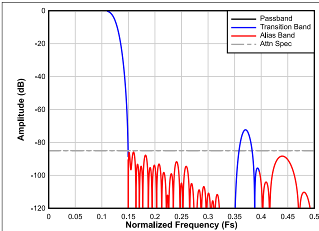
Figure 7-21. Complex Decimation by 4 Filter Response
