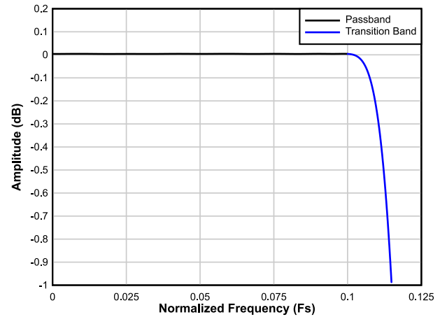
Figure 7-22. Decimation by 4 Passband Ripple Response
