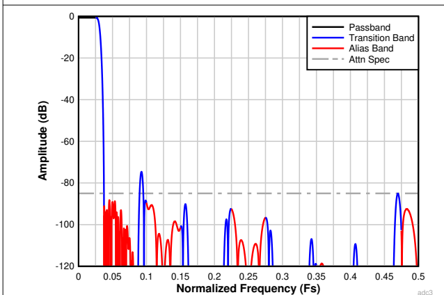
Figure 7-25. Complex Decimation by 16 Filter Response
