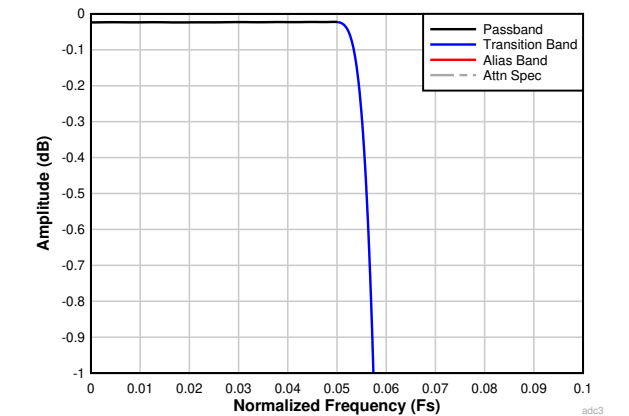
Figure 7-24. Decimation by 8 Passband Ripple Response
