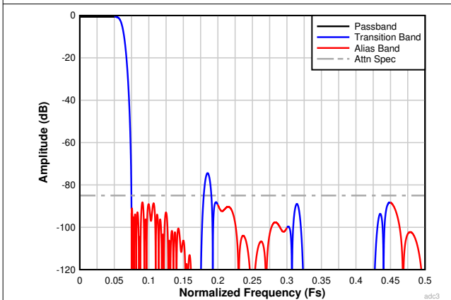
Figure 7-23. Complex Decimation by 8 Filter Response
