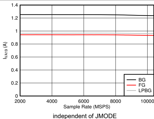
Figure 5-121. DES Mode: I_{VA19} vs Sample Rate
