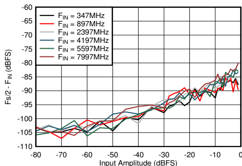
Figure 5-79. Dual Channel Mode: F_s/2 - F_{\text{IN}} vs Input Amplitude and Frequency
