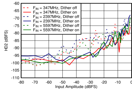
Figure 5-64. DES Mode: HD2 vs Input Amplitude and Dither
