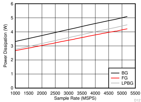
Figure 5-139. Dual Channel Mode: Power Dissipation vs Sample Rate
