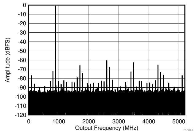
Figure 5-6. DES Mode: Single Tone FFT at 897MHz
