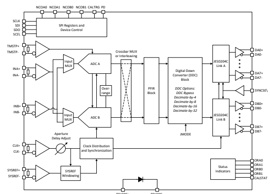
ADC12DJ5200-SP Block Diagram
