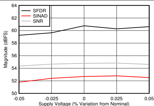
Figure 5-95. DES Mode: SNR, SINAD and SFDR vs Supply Voltage
