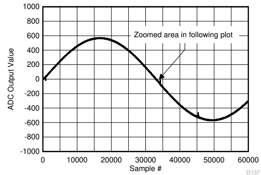
Figure 5-144. Background Calibration Core Transition (AC Signal)
