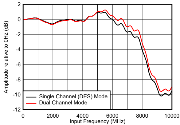
Figure 5-1. Input Amplitude vs Input Frequency
