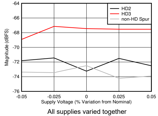
Figure 5-98. Dual Channel Mode: HD2, HD3 and Worst non-HD Spur vs Supply Voltage
