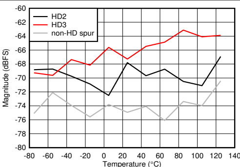
Figure 5-89. DES Mode: HD2, HD3 and Worst non-HD Spur vs Temperature
