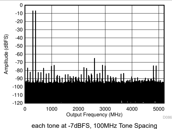
Figure 5-11. DES Mode: Two Tone FFT at 347MHz
