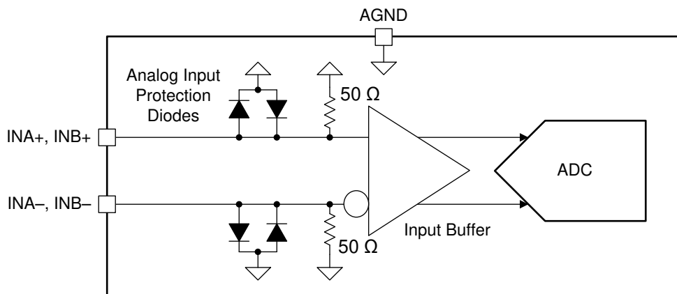
Figure 6-1. ADC12DJ5200-SP Analog Input Internal Termination and Protection Diagram
