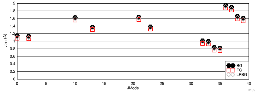
Figure 5-120. Other Modes with Lower Maximum F_S : I_{VA11} vs JMODE
