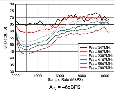
Figure 5-33. DES Mode: SFDR vs Sample Rate and Input Frequency
