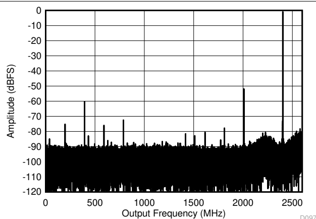
Figure 5-22. Dual Channel Mode: Single Tone FFT at 7997MHz
