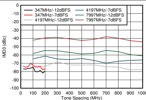
Figure 5-108. Dual Channel Mode: IMD3 vs Tone Spacing
