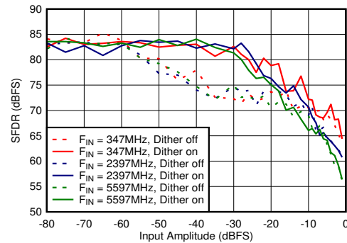
Figure 5-62. DES Mode: SFDR vs Input Amplitude and Dither
