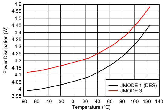
Figure 5-143. Power Dissipation vs Temperature
