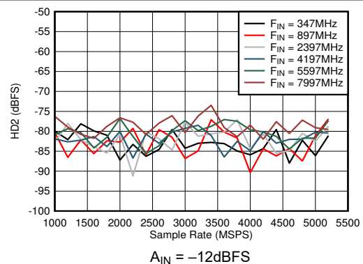
Figure 5-54. Dual Channel Mode: HD2 vs Sample Rate and Input Frequency
