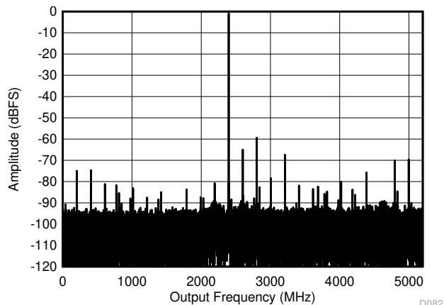
Figure 5-7. DES Mode: Single Tone FFT at 2397MHz
