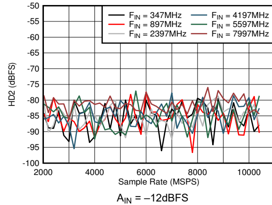
Figure 5-38. DES Mode: HD2 vs Sample Rate and Input Frequency
