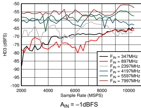
Figure 5-39. DES Mode: HD3 vs Sample Rate and Input Frequency
