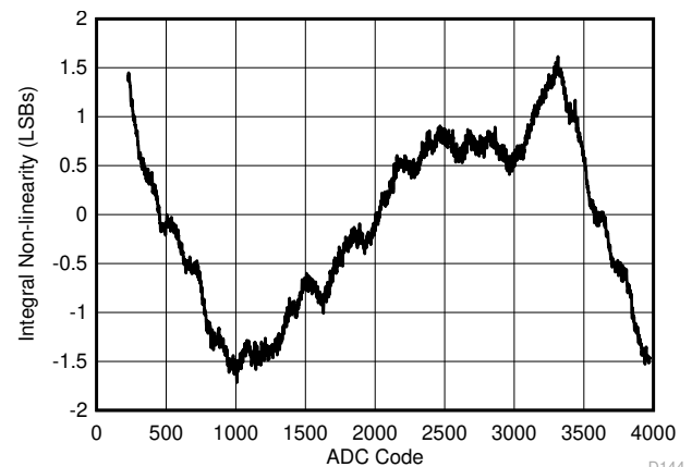
Figure 5-4. INL vs ADC Code
