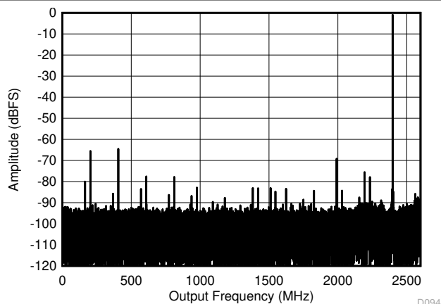
Figure 5-19. Dual Channel Mode: Single Tone FFT at 2397MHz
