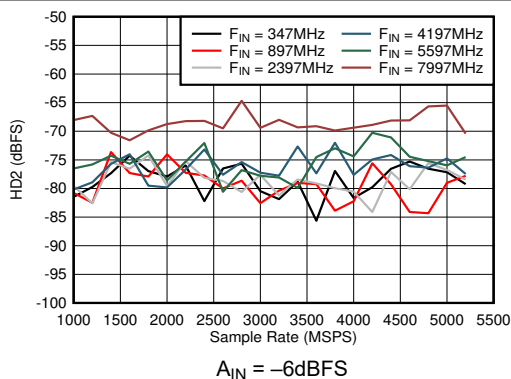
Figure 5-53. Dual Channel Mode: HD2 vs Sample Rate and Input Frequency
