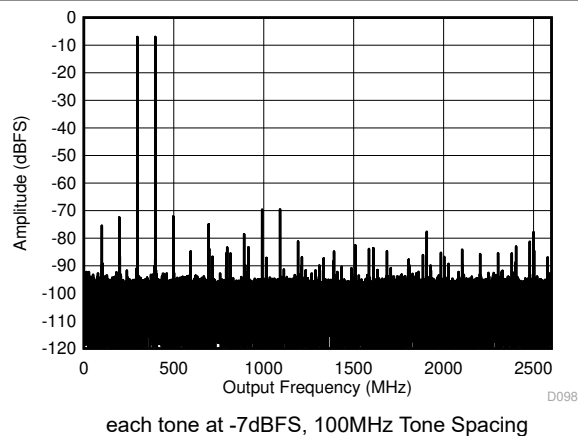
Figure 5-23. Dual Channel Mode: Two Tone FFT at 347MHz
