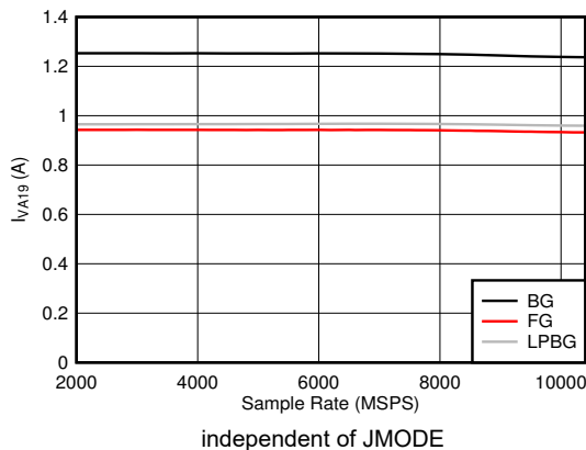
Figure 5-123. DES Mode: I_{VA19} vs Sample Rate
