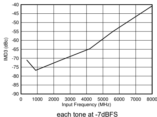
Figure 5-106. Dual Channel Mode: IMD3 vs Input Frequency
