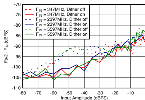
Figure 5-82. Dual Channel Mode: F_s/2 - F_{\text{IN}} vs Input Amplitude and Dither
