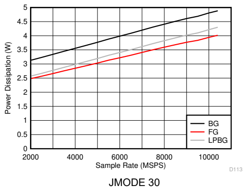
Figure 5-131. DES Mode: Power Dissipation vs Sample Rate
