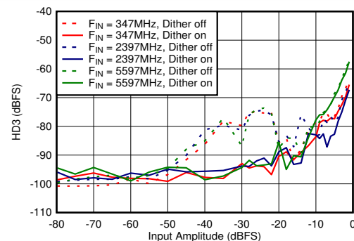
Figure 5-66. DES Mode: HD3 vs Input Amplitude and Dither
