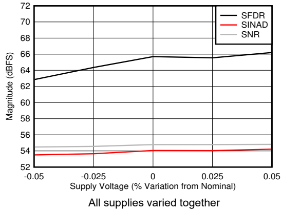
Figure 5-97. Dual Channel Mode: SNR, SINAD and SFDR vs Supply Voltage
