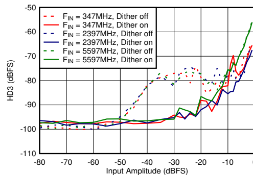
Figure 5-80. Dual Channel Mode: HD3 vs Input Amplitude and Dither
