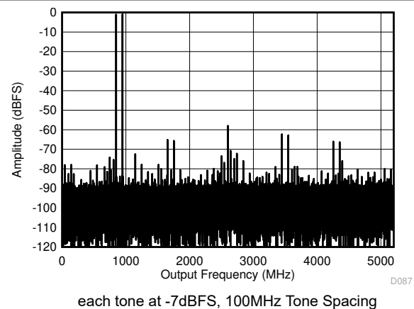
Figure 5-12. DES Mode: Two Tone FFT at 897MHz
