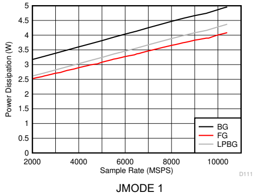
Figure 5-129. DES Mode: Power Dissipation vs Sample Rate
