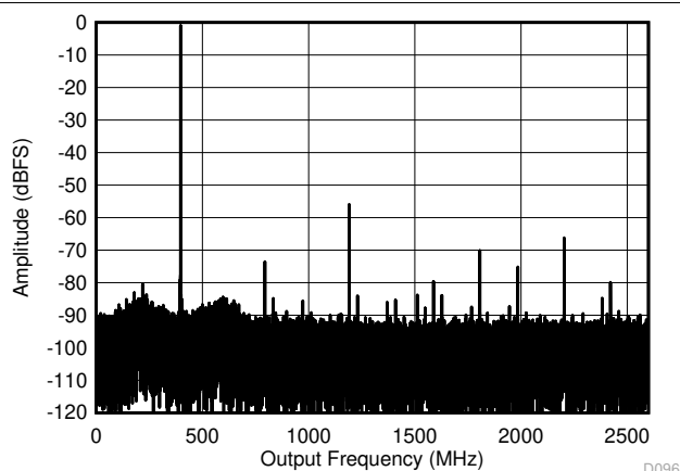
Figure 5-21. Dual Channel Mode: Single Tone FFT at 5597MHz
