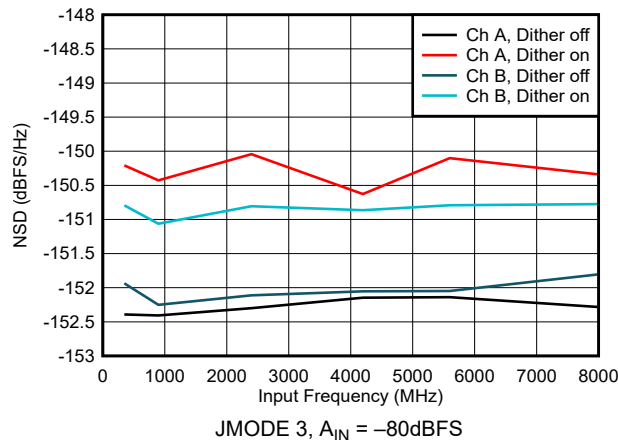
Figure 5-51. Dual Channel Mode: NSD and Input Frequency
