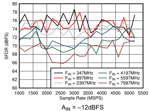
Figure 5-50. Dual Channel Mode: SFDR vs Sample Rate and Input Frequency
