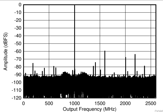
Figure 5-20. Dual Channel Mode: Single Tone FFT at 4197MHz
