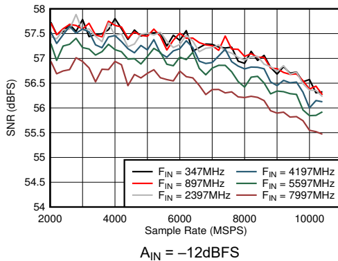
Figure 5-31. DES Mode: SNR vs Sample Rate and Input Frequency
