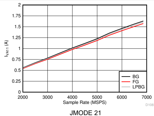
Figure 5-126. DES Mode: I_{VD11} vs Sample Rate
