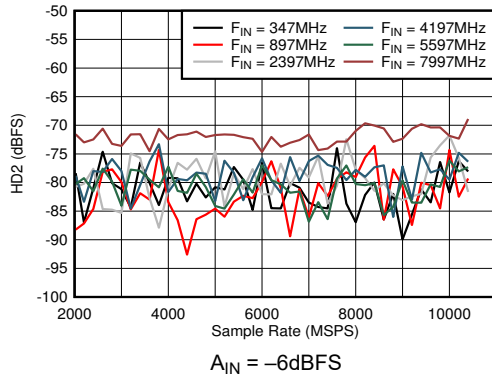
Figure 5-37. DES Mode: HD2 vs Sample Rate and Input Frequency
