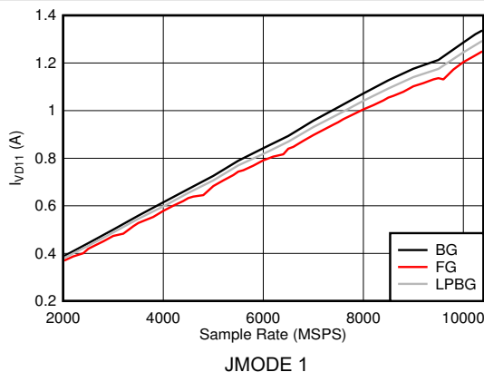
Figure 5-125. DES Mode: I_{VD11} vs Sample Rate
