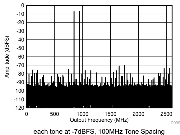
Figure 5-24. Dual Channel Mode: Two Tone FFT at 897MHz
