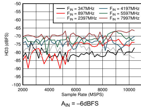
Figure 5-40. DES Mode: HD3 vs Sample Rate and Input Frequency
