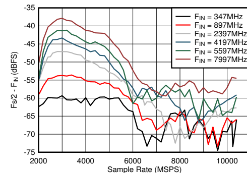
Figure 5-42. DES Mode: F_{\text{s}}/2 - F_{\text{IN}} vs Sample Rate and Input Frequency
