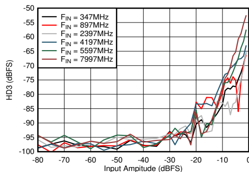
Figure 5-65. DES Mode: HD3 vs Input Amplitude and Frequency
