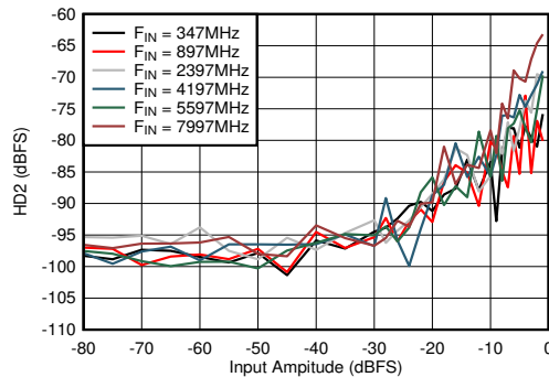
Figure 5-63. DES Mode: HD2 vs Input Amplitude and Frequency
