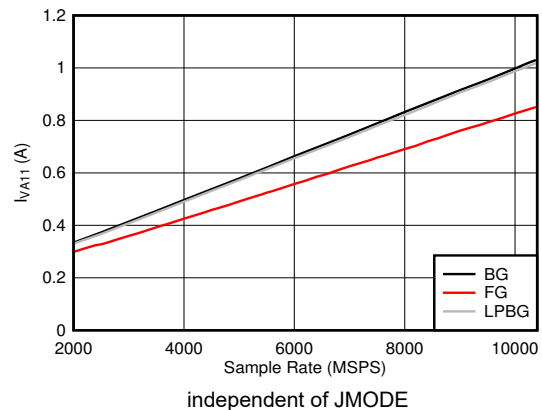
Figure 5-124. DES Mode: I_{VA11} vs Sample Rate
