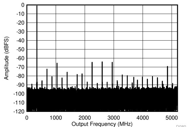
Figure 5-5. DES Mode: Single Tone FFT at 347 MHz
