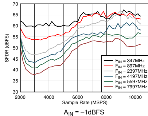
Figure 5-32. DES Mode: SFDR vs Sample Rate and Input Frequency
