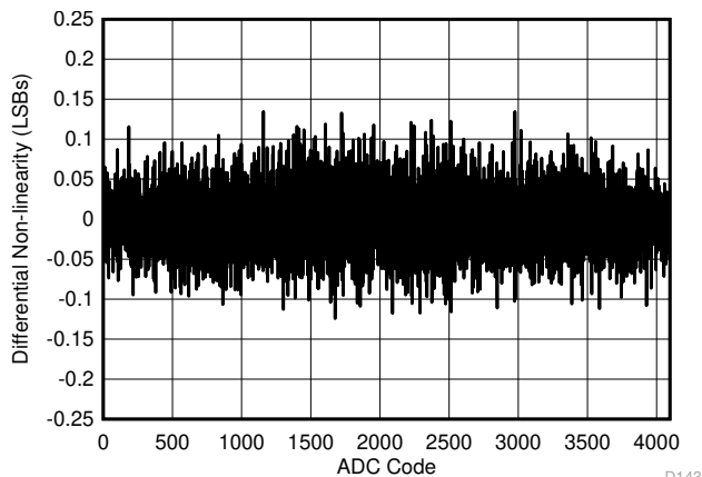
Figure 5-3. DNL vs ADC Code
