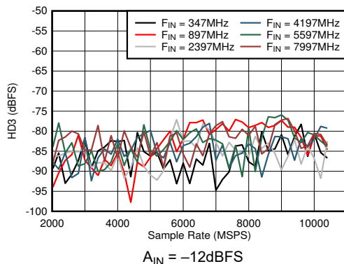
Figure 5-41. DES Mode: HD3 vs Sample Rate and Input Frequency
