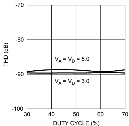
Figure 18. THD vs SCLK Duty Cycle
