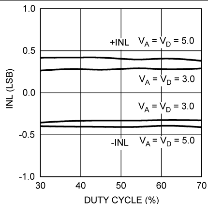
Figure 16. INL vs SCLK Duty Cycle
